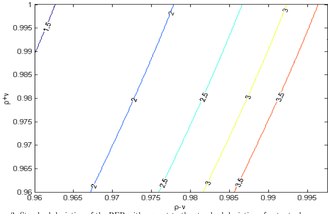
Figure 3: Standard deviation of the RER with respect to the standard deviation of output when \rho and \nu change
