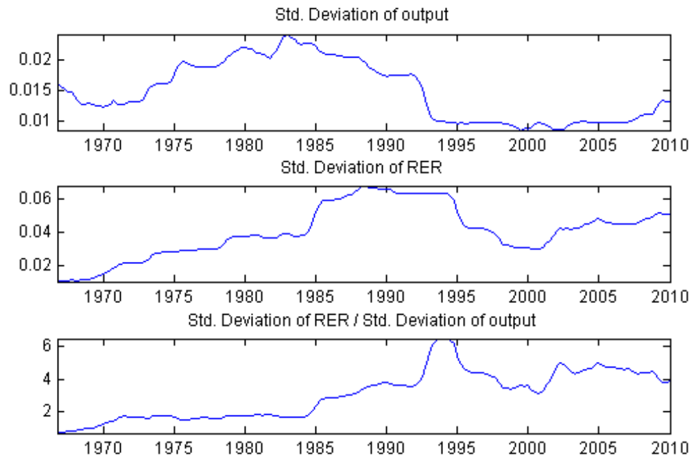
Figure 1: Standard deviation of HP-filtered output and RER and the ratio of standard deviations
