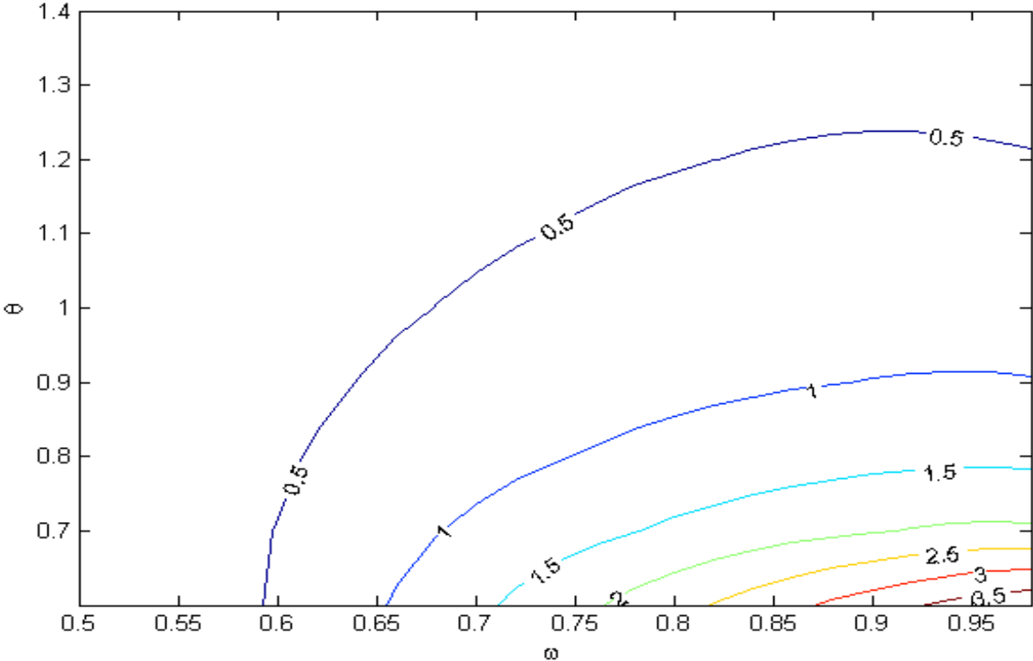
Figure 2: Standard deviation of the RER with respect to the standard deviation of output when \theta and \omega change
